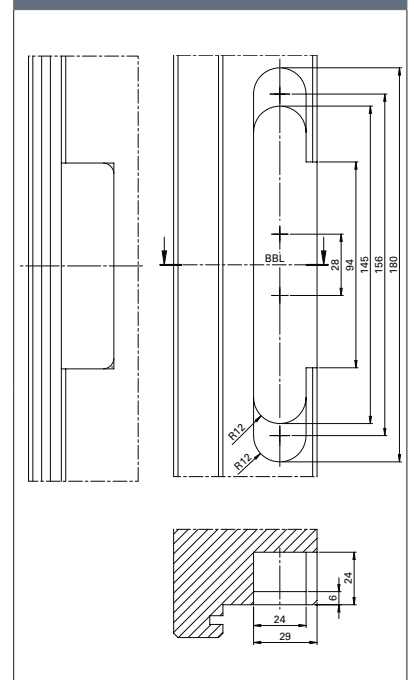
Milling pattern with cover bracket
