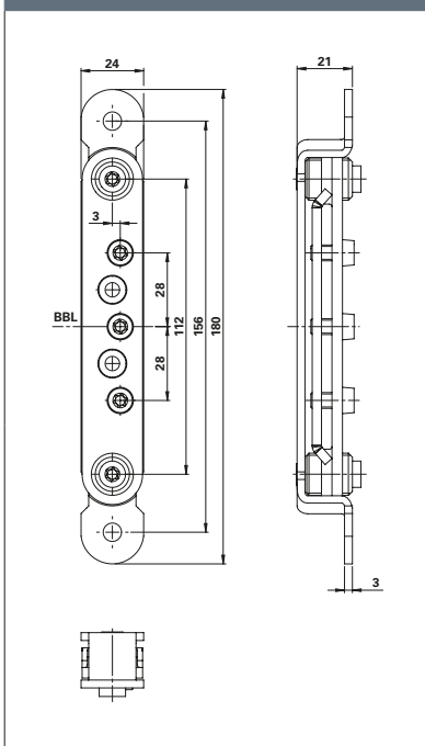
Dimensional drawing
