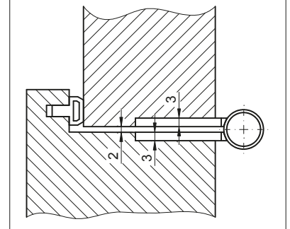
Cross-section
