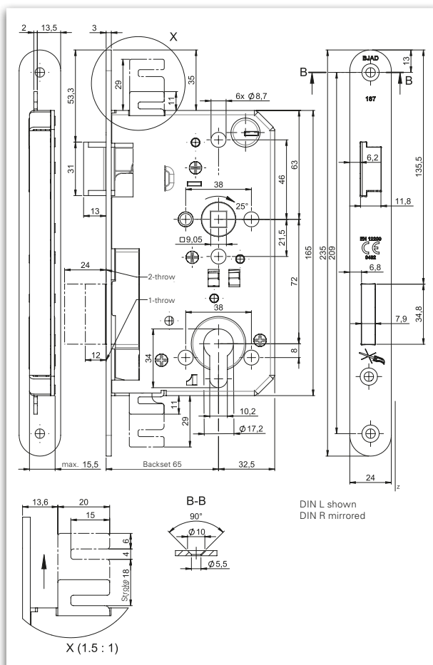
Dimensions: GBS 187
