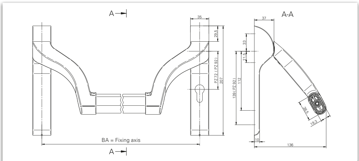
Dimensions: Guardian EPN 900 IV with security short plate counter fitting
