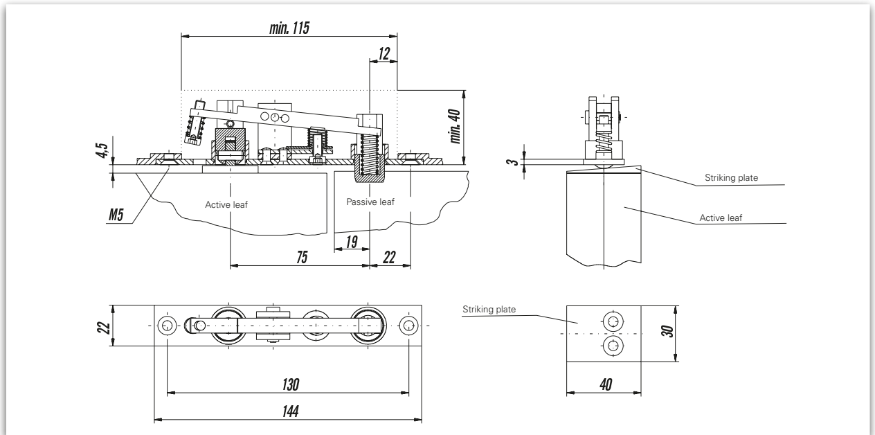
Dimensions: Dual locking system 1 with roller latch
