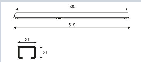
Slide rail ECO IS 21
