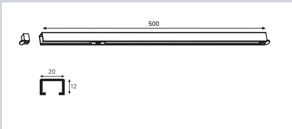
Slide rail ECO IS 12
